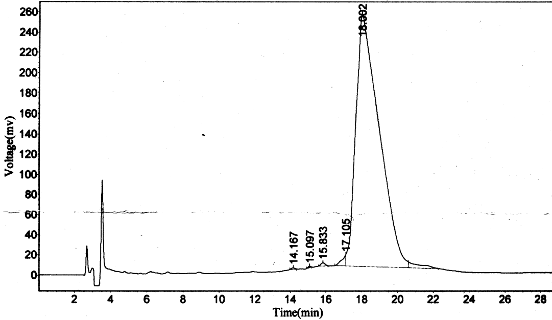
Chromatogram (AF-30-2-3-F-050512.mdy)
