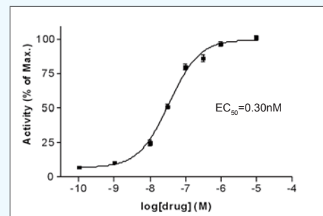
Fig 2 Carbachol dose response of HEK293/M1R cell line with detection of intracellular calcium flux.
