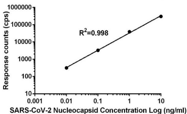
LFA Analysis with A02135 (N338) as capture antibody and A02136 (N34) as detection antibody
